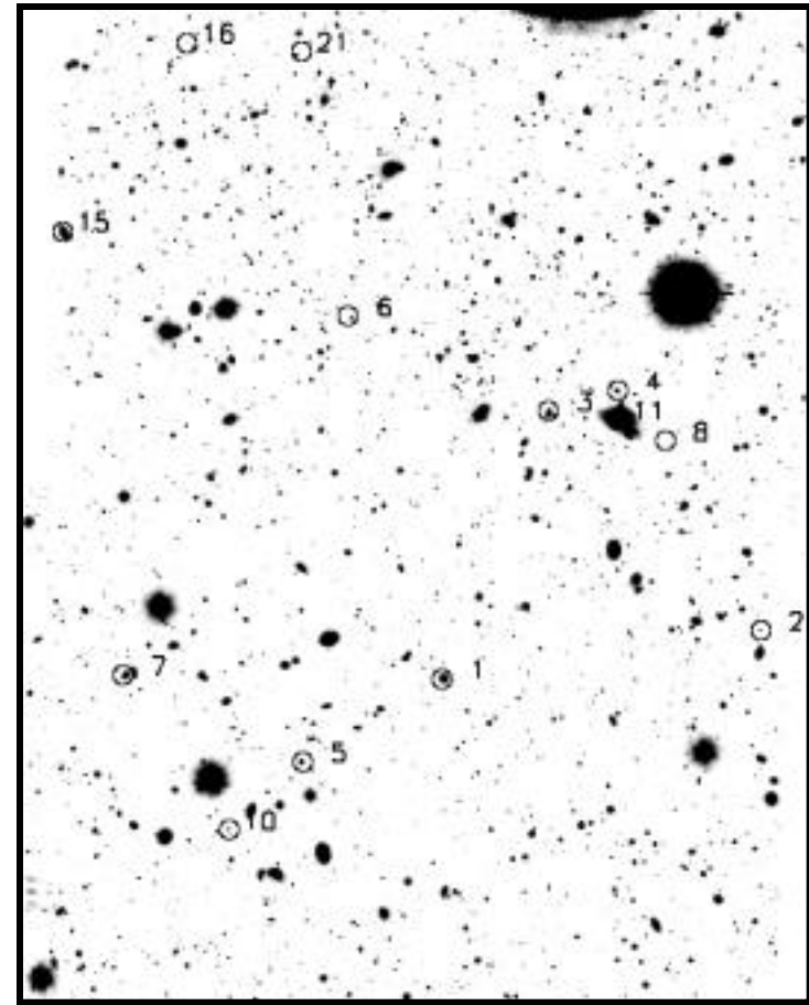
Deep Optical with X-Ray Contours
