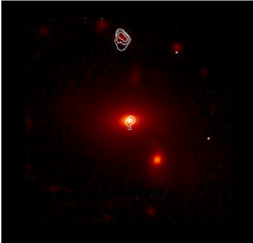
Optical with X-Ray Contours
