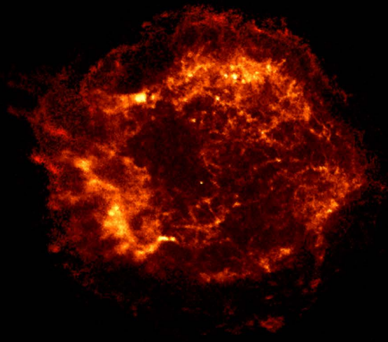
X-Ray (NASA/CXC/SAO)
