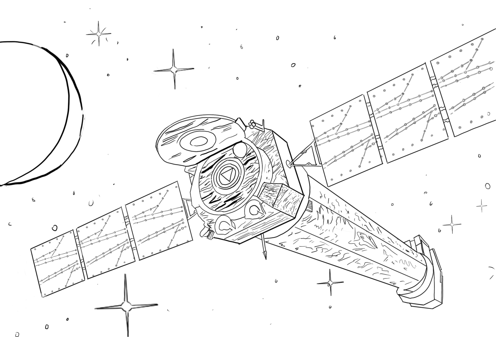
Chandra X-Ray Observatory
